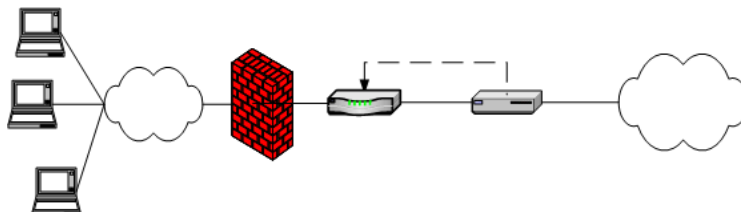
Pulse Connect Secure and IDP Topology Scenario 2
